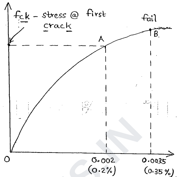
■ Original \sigma - \epsilon curve of concrete.
