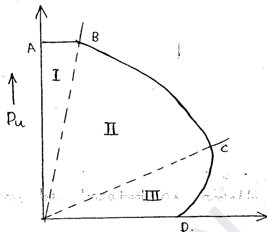
Interaction Curve (SP 16)
