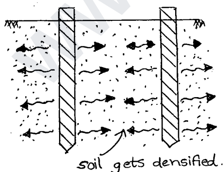
■ Compaction pile.
