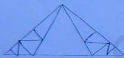
Compound fink
