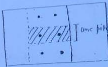
Double rivetted lap joint
